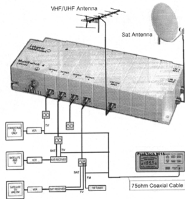
Fig. 3-1 Connecting with LNB
